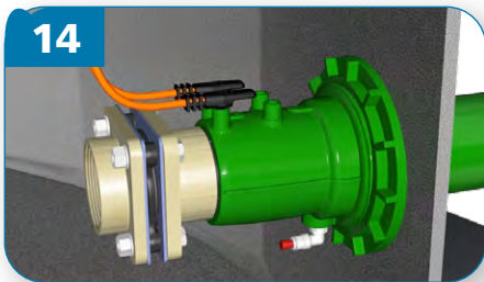
14 Mount the fitting, connect the welding cables and weld.
