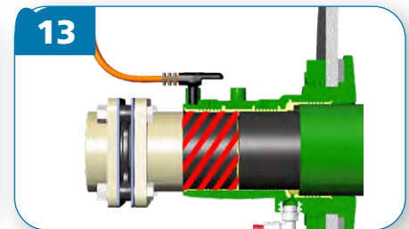
13 When welding the fitting, the outer welding towers should be used. Add a KP CC in the joint.
