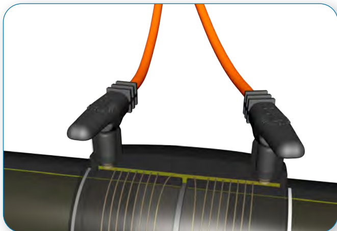
During electrofusion welding material is melted by the heat from the socket wiring and the pipe fuses with the welding socket.
