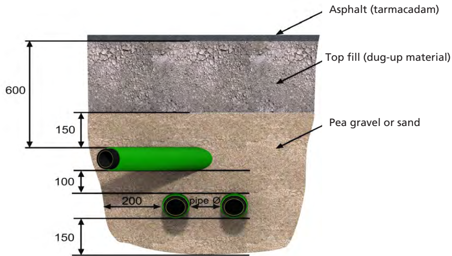
Minimum clearances for vehicles weighing up to 60 tons.
