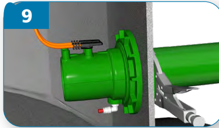
9 Mount and make sure the pipes are in position. Connect the welding cables and follow the welding machine instructions.
