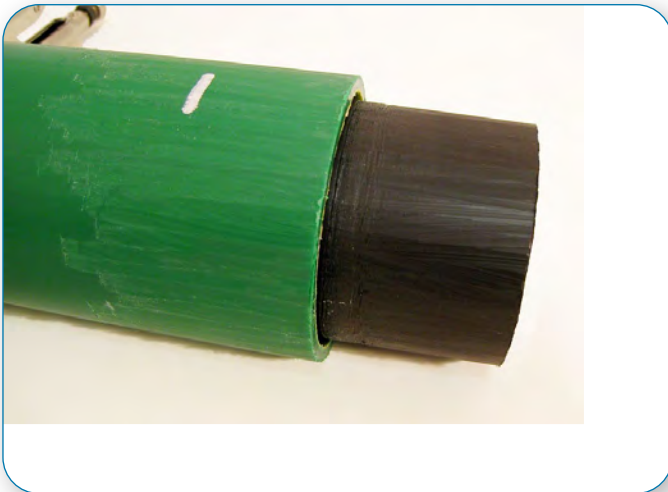
Correctly scraped pipes. Oxide has been removed from the whole area to be welded.
