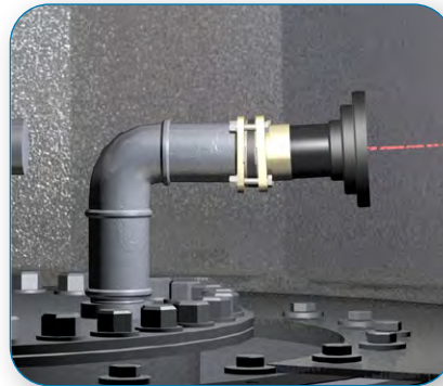
Place the laser pointer in the pre-mounted fittings on the manway lid.
