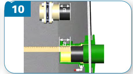
10 Measure the insert depth and mark it on the transition fitting.
